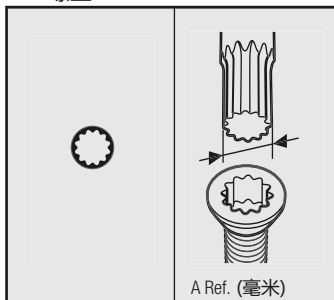
XZN 螺丝
