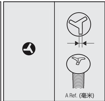
TRI-WING® 螺丝
