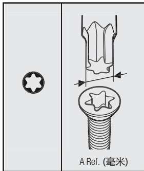
TORX® 螺丝
